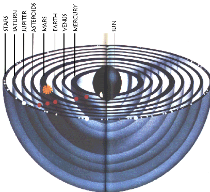
The Solar System Onion
